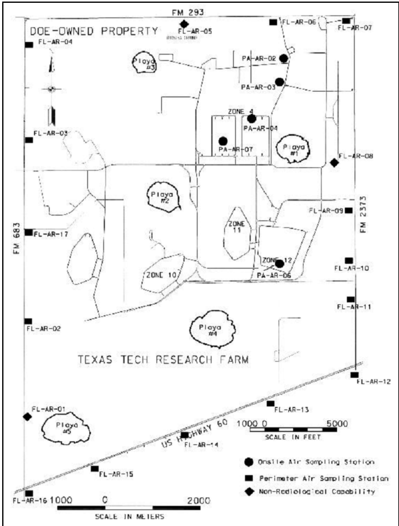
Figure 4-3. Air monitoring stations in 2000 (DOE 2001a)
