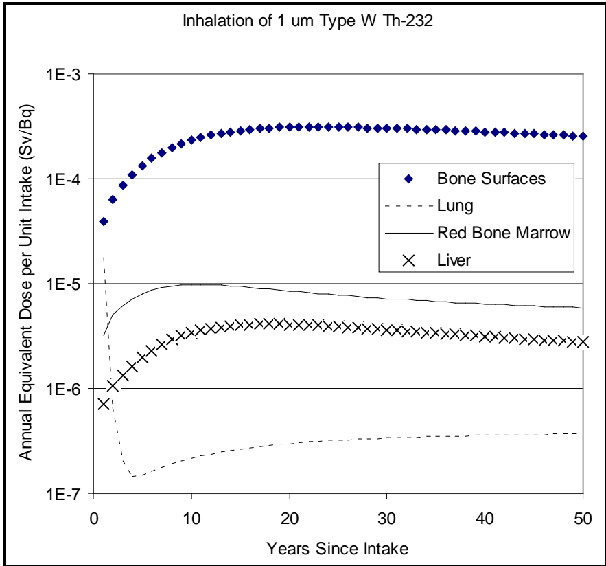
Figure 4-7. IMBA (OCAS 2003) equivalent dose to four tissues or organs per unit intake (Sv/Bq) during each year for 1-μm AMAD Type W 232 Th inhalation.
