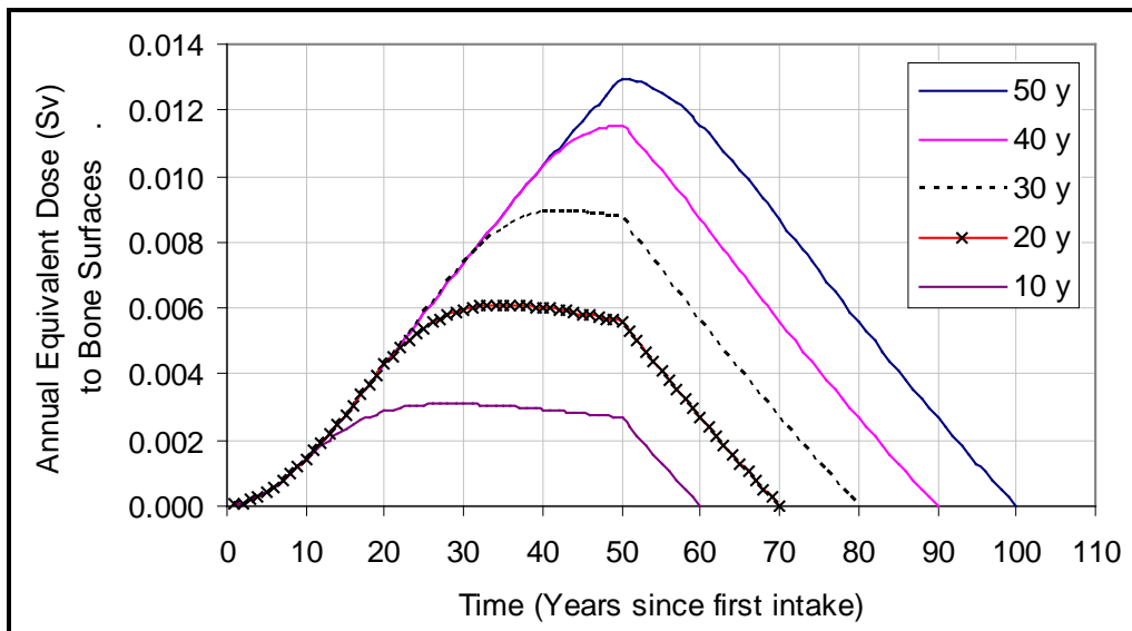
Figure 4-9. IMBA (OCAS 2003) annual equivalent dose (Sv) to bone surfaces for 10, 20, 30, 40, and 50-year inhalation intakes of 1 Bq per year of 1 \mu\text{m} Type W ^{232}\text{Th} .
