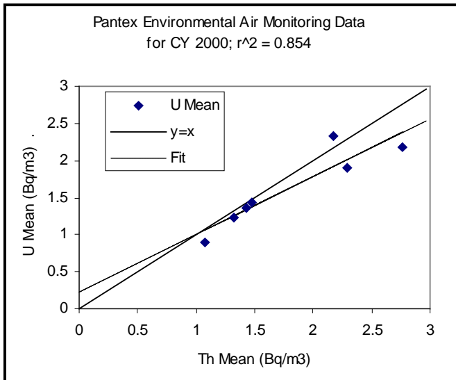
Figure 4-5. Pantex ^{238}\text{U} and thorium mean environmental air monitoring data for 2000 at seven locations.
