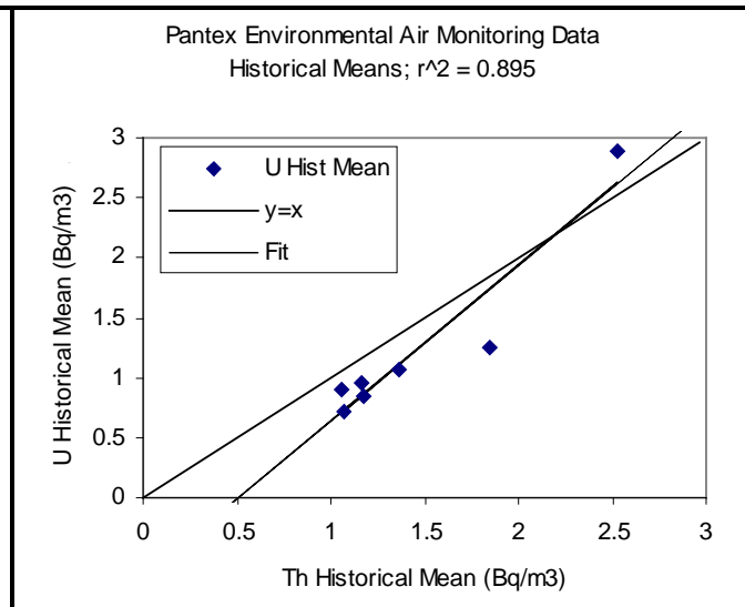
Figure 4-6. Pantex ^{238}\text{U} and thorium mean environmental air monitoring data (historic) at seven locations.
