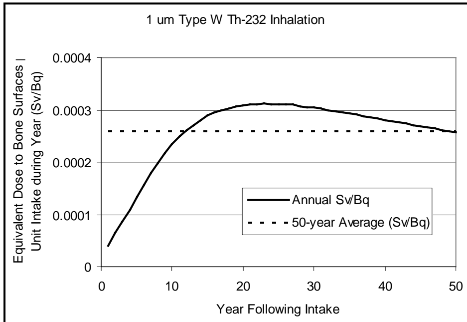
Figure 4-8. IMBA (OCAS 2003) equivalent dose and average equivalent dose to bone surfaces per unit intake (Sv/Bq) during each year for 1 \mu\text{m} AMAD Type W ^{232}\text{Th} inhalation.
