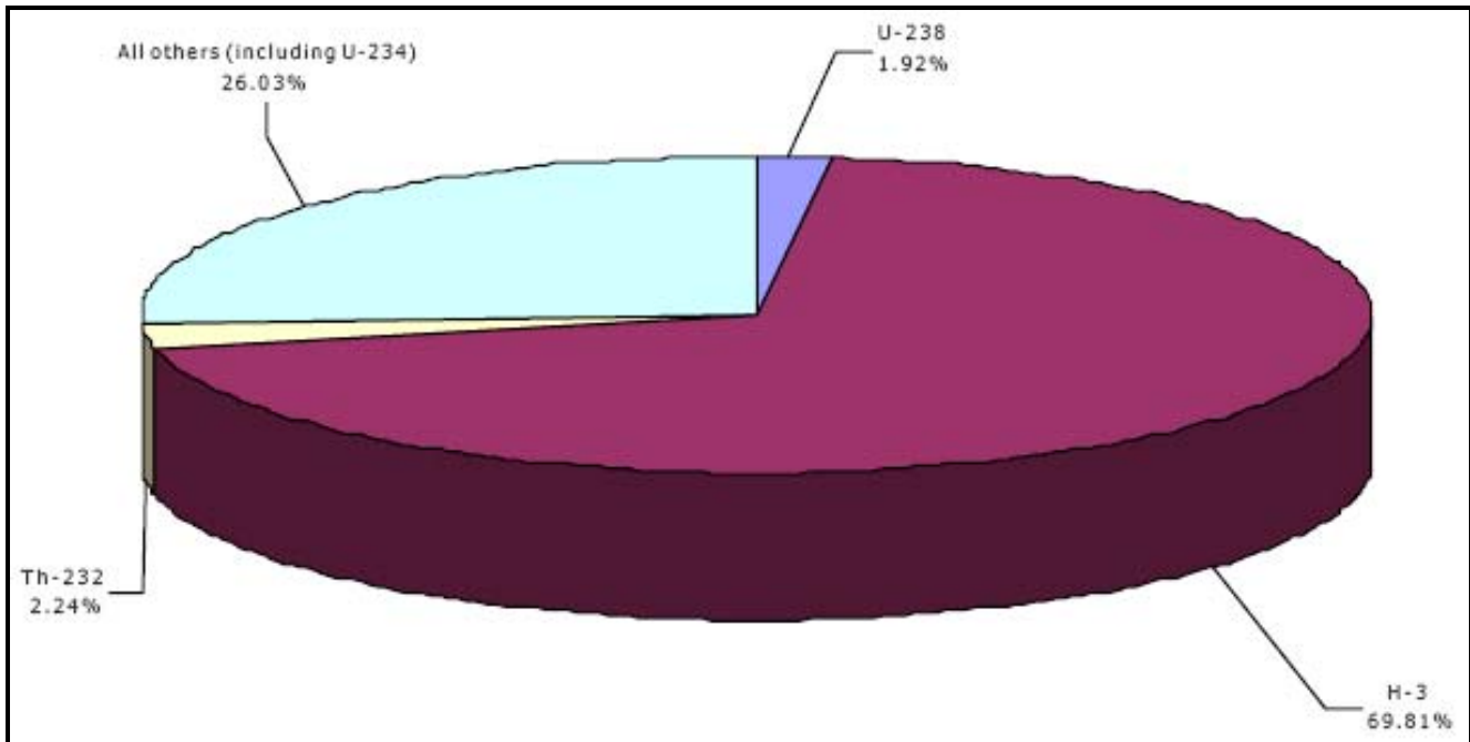
Figure 4-2. Isotopic contributions to offsite dose from Pantex operations in 2000 (DOE 2001a).
