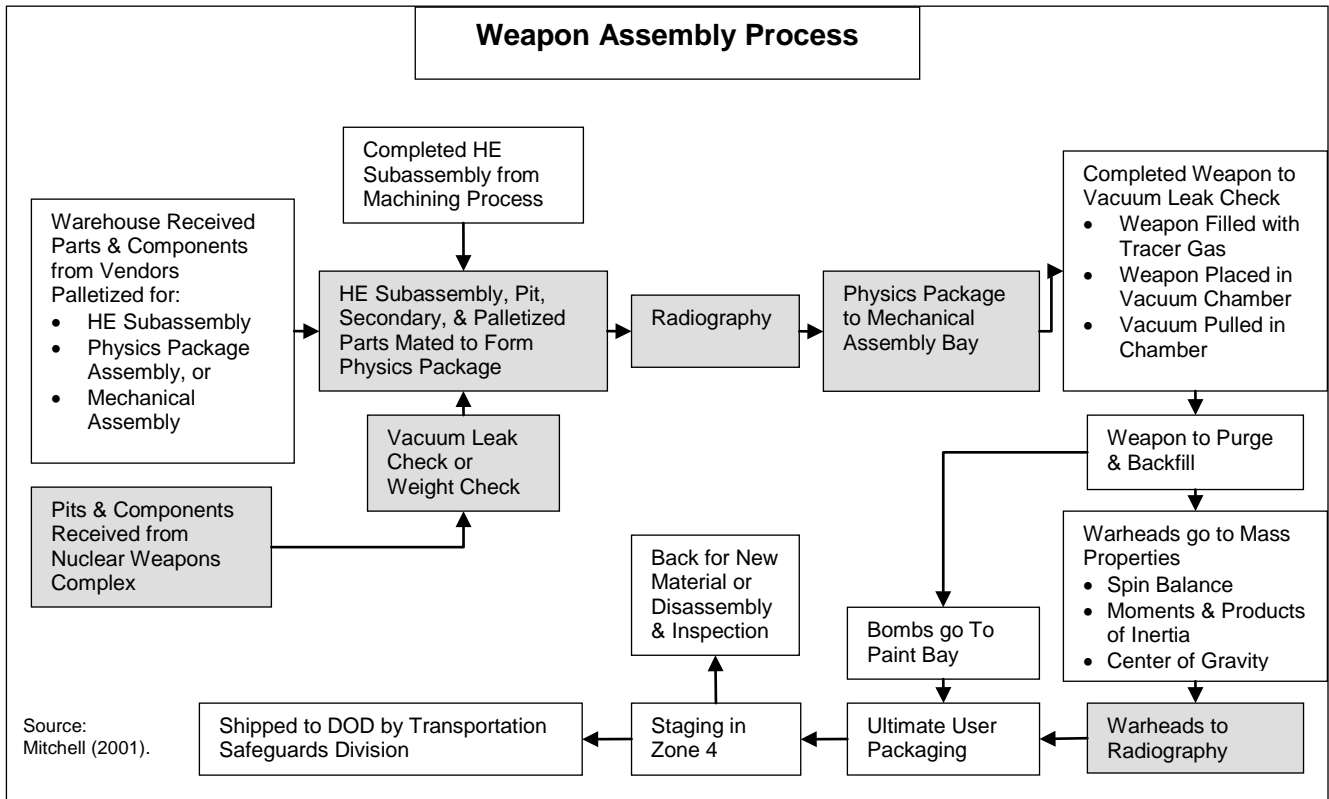
Figure 2-2. Pantex nuclear weapon assembly process.
