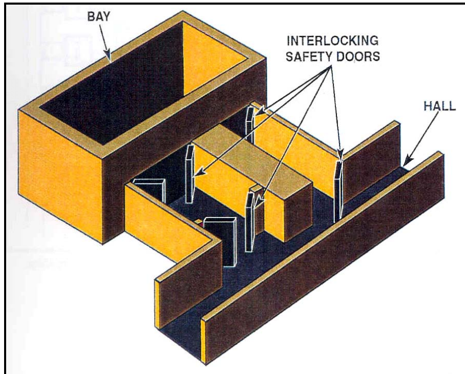
Figure 2-4. Generic representation of a nuclear explosive bay.
