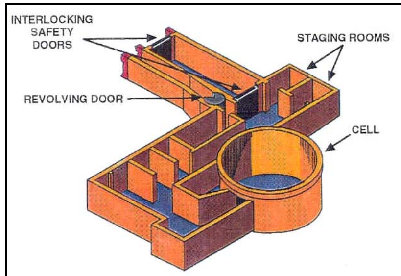
Figure 2-5. Generic representation of a nuclear explosive cell.
