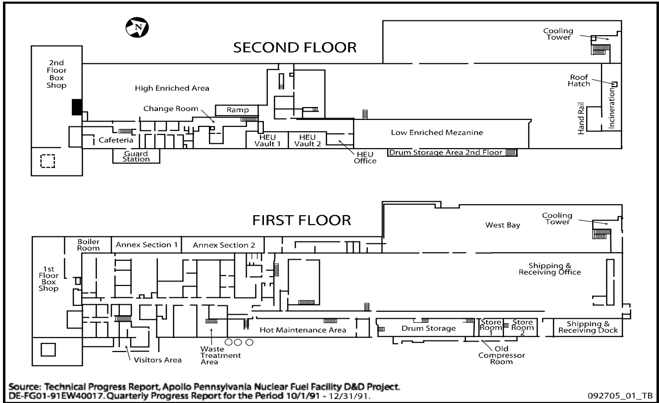
Figure 2-2. Site floor plan at NUMEC Apollo.
