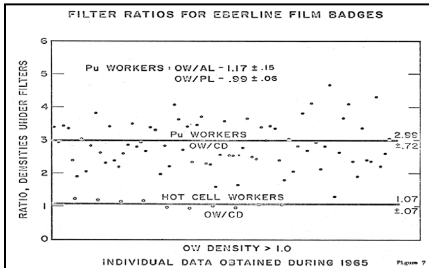
Figure 6-3. Dosimeter filter ratios (Caldwell 1966b).
