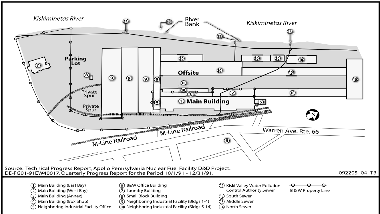
Figure 2-1. Site layout, NUMEC Apollo.
