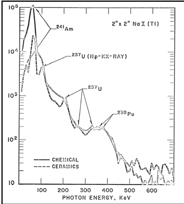
Figure 6-1. Gamma spectrum external to plutonium chemical processing line and plutonium ceramics line (Caldwell 1966b, figure 3).
