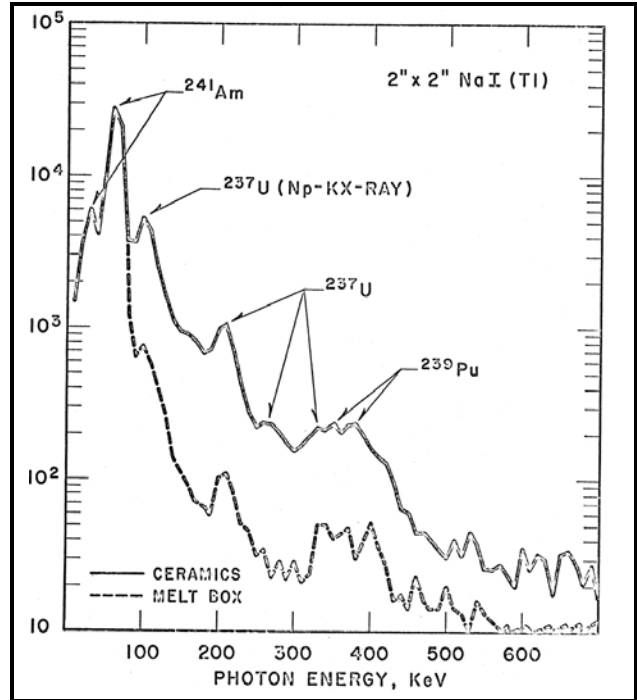
Figure 6-2. Gamma spectrum external to plutonium ceramics line and plutonium melt glovebox (Caldwell 1966b, figure 4).
