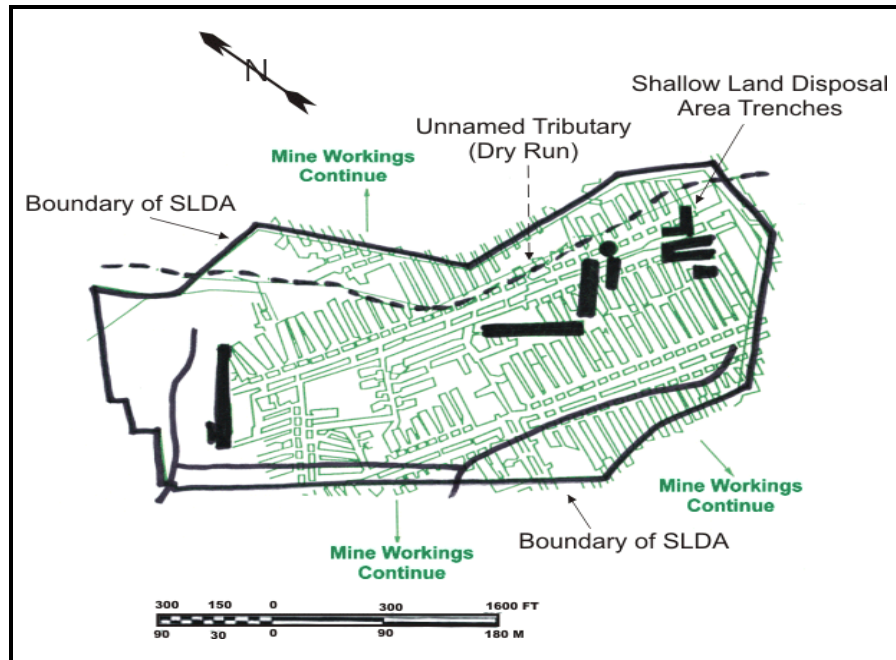
Figure 2-4. B&W Shallow Land Disposal Area (SLDA) (USAEC 2007).
