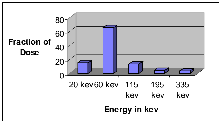
Figure 6-4. Relative contribution by energy group to personnel exposure during plutonium fuel fabrication from 1000 MWD/T plutonium (Caldwell 1966b, p. 18, Figure 8).
