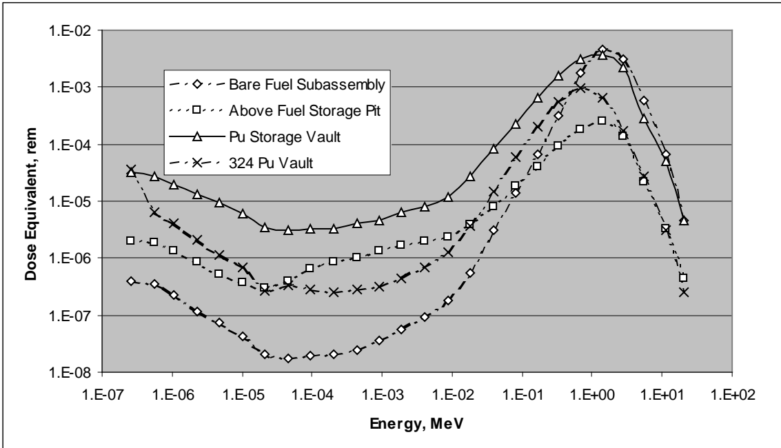
Figure 6.3.4.5-3. Neutron spectra for Hanford 308 and 324 facilities. (Fix et al 1982)
