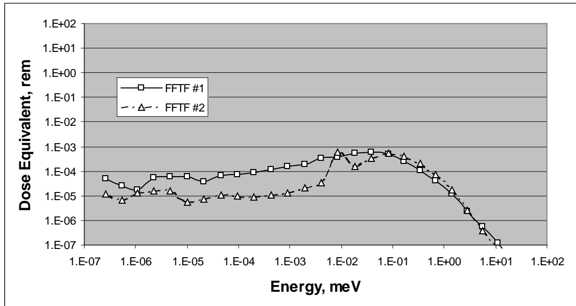
Figure 6.3.4.5-4. Neutron spectra for Hanford 400 Area FFTF.
