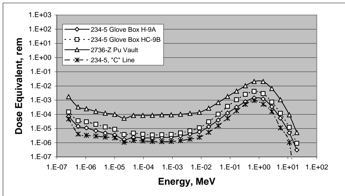
Figure 6.3.4.5-2. Neutron energy spectra recorded at Hanford PFP 234-5Z "C" line, glovebox and plutonium storage vault.
