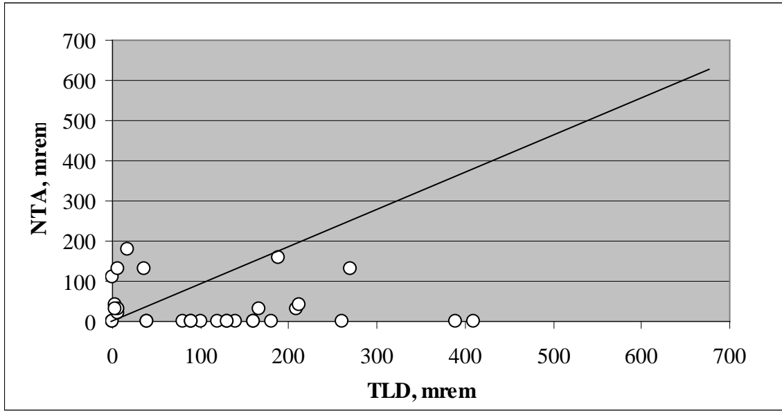
Figure 6.3.4.4-1. Comparison of Hanford PFP workplace NTA and HMPD neutron dose. (Nichols et al 1972)
