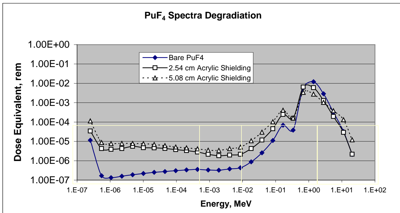
Figure 6.3.4.5-1. Degradation in neutron energy spectra for bare, 2.54 cm and 5.08 cm of acrylic plastic shielding with neutron energy groups overlay.
