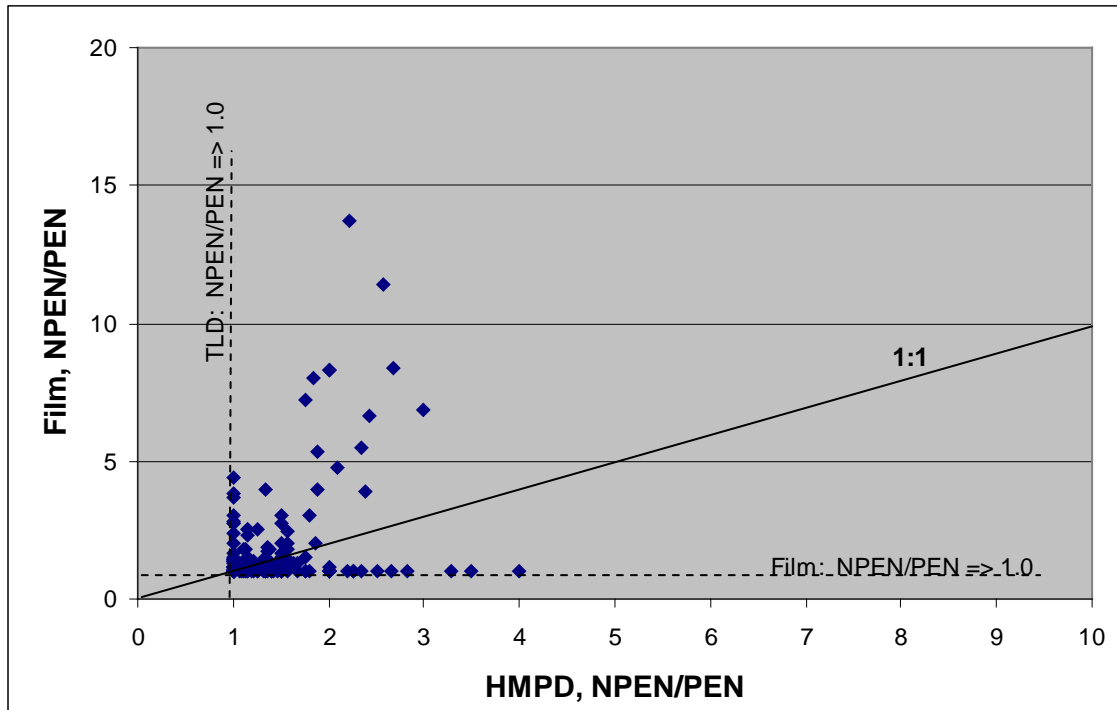
Figure 6.3.4.2-1. Ratio of nonpenetrating (NPEN) to penetrating (PEN) dose for HMPD and film parallel workplace measurements.
