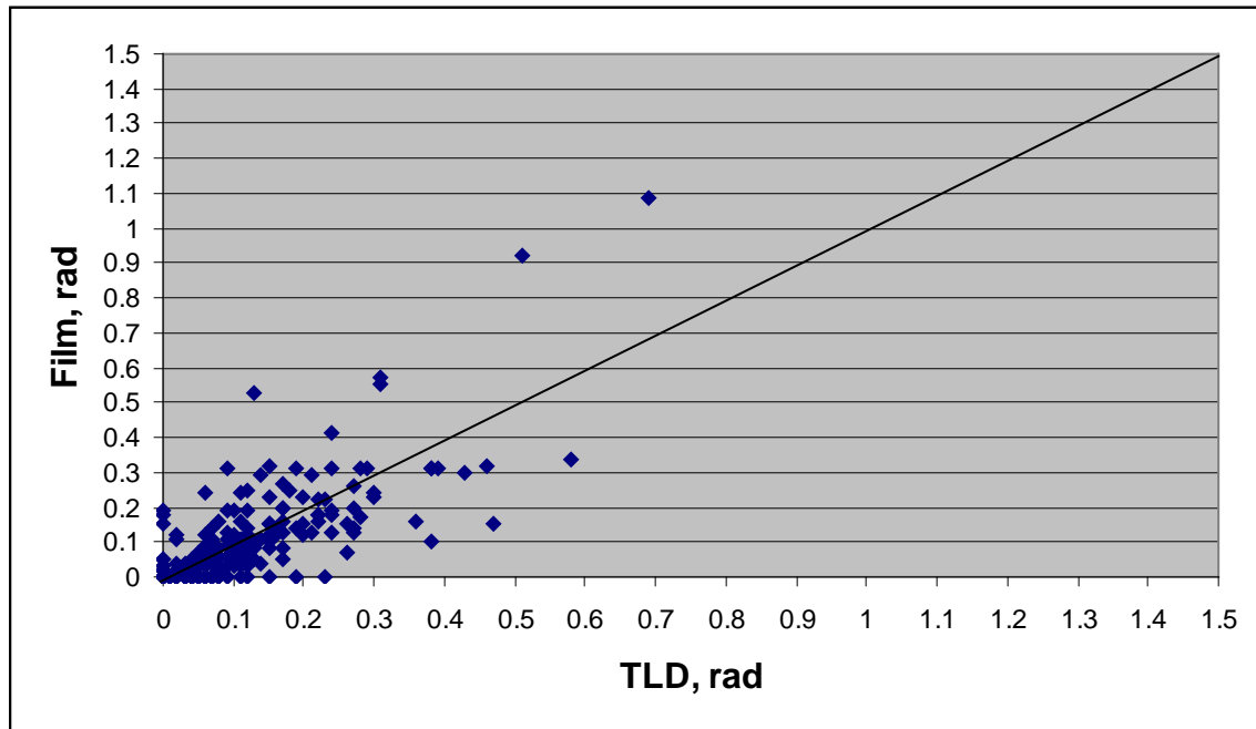
Figure 6.3.4.1-2. Comparison of Hanford film and TLD nonpenetrating dose results. (Nichols et al 1972)
