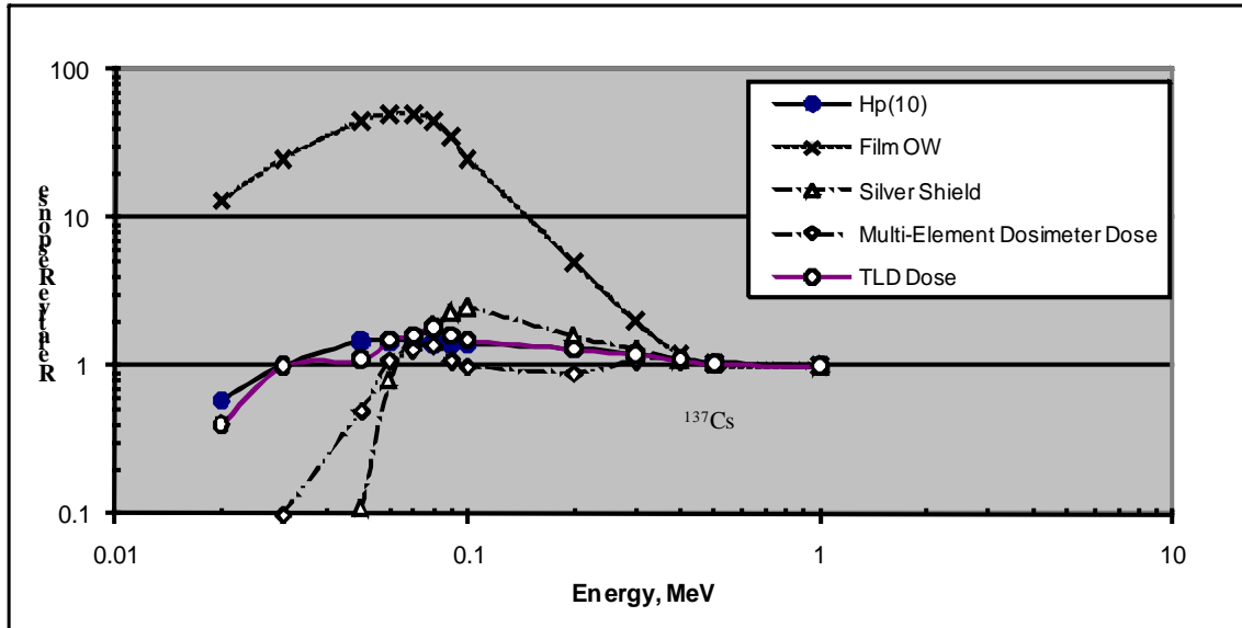
Figure 6.3.3.1-1. Measured Hanford dosimeter photon response characteristics. (Wilson et al 1990)
