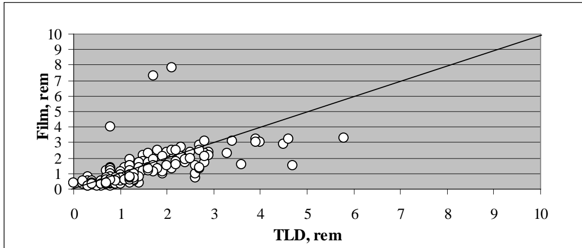
Figure 6.3.4.1-1. Comparison of Hanford film and TLD penetrating dose results. (Nichols et al 1972)
