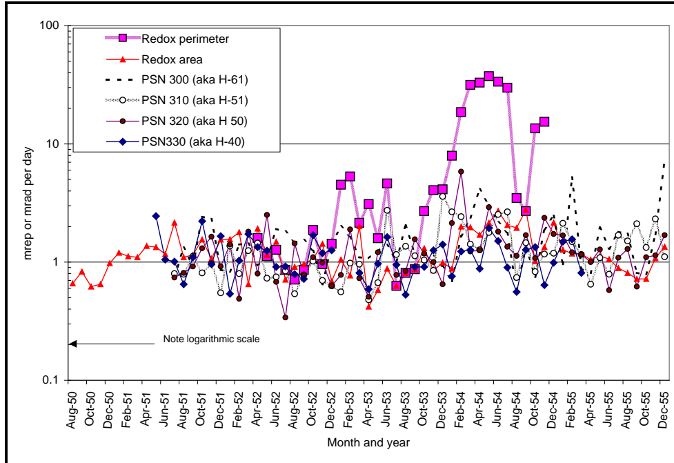
Figure 4.3.1-2. Exposure rates measured near the REDOX Plant and at four military installations. Measured exposure rates at the REDOX perimeter are the highest of all environmental stations monitored between 1945 and 1955. Monitoring at the perimeter was discontinued in December 1954, although monitoring continued in the REDOX area (Till et al. 2002)
