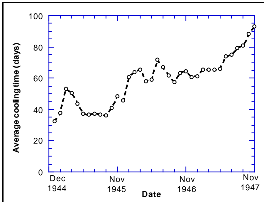
Figure 4.2.1-1. Average fuel cooling times prior to processing at Hanford.
