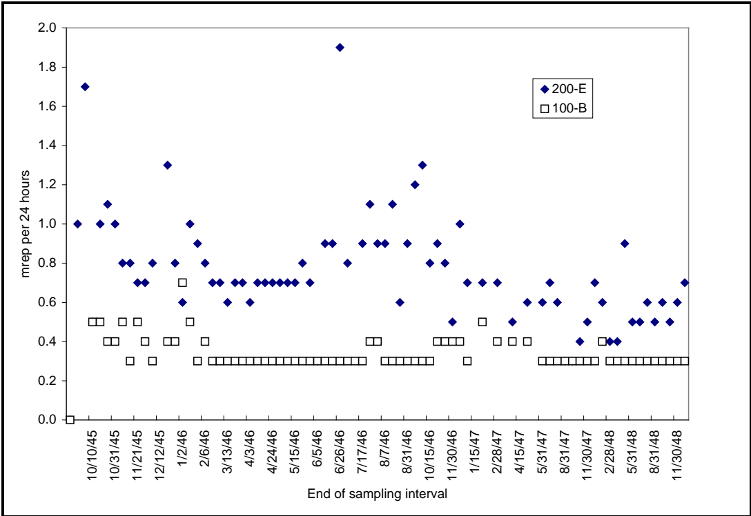
Figure 4.3.1-1. Radiation levels measured by detachable C chambers at two locations on the Hanford Site, 1945–1948. Levels at 200-East (separations area) averaged roughly twice those at 100-B (a reactor area). The average level at 100-B was 0.35 mrep per 24 hours, which is within the stated background range of the instrument (0.3–0.5 mrep per 24 hours), and the average level at 200-East was 0.75 mrep per 24 hours (data from HW-9871) (Till et al. 2002).
