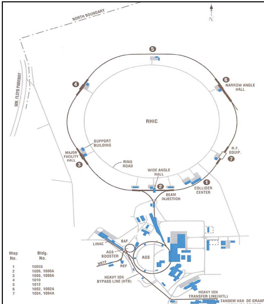
Figure 2-4. The Relativistic Heavy Ion Collider (RHIC) Complex.
