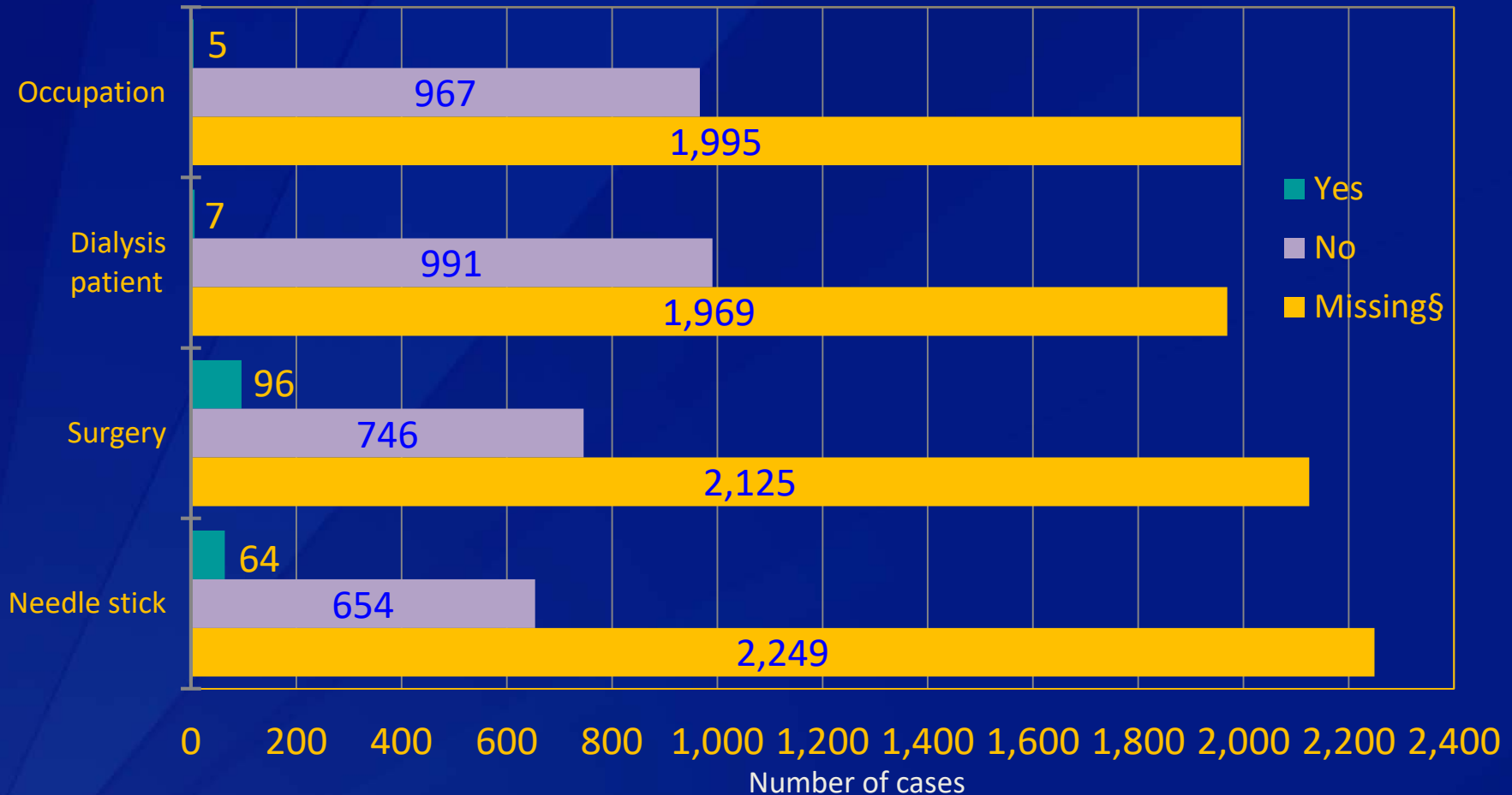
Figure 4.6b. Acute hepatitis C reports*, by risk exposure/behavior† — United States, 2016
