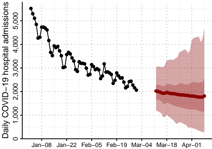
Ensemble forecast
