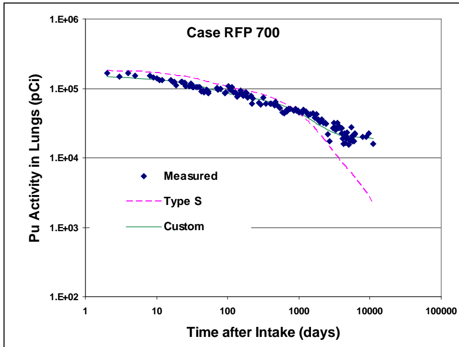
Figure A-7. Comparison of Type S and custom models for Case RFP 700.
