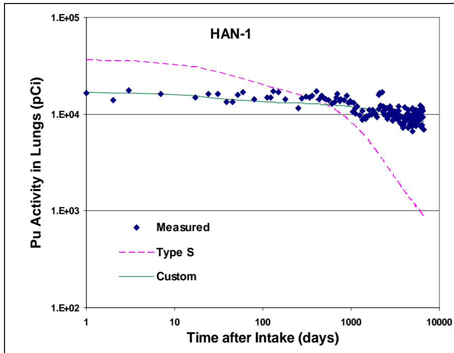
Figure A-10. Comparison of Type S and custom models for Case HAN-1.
