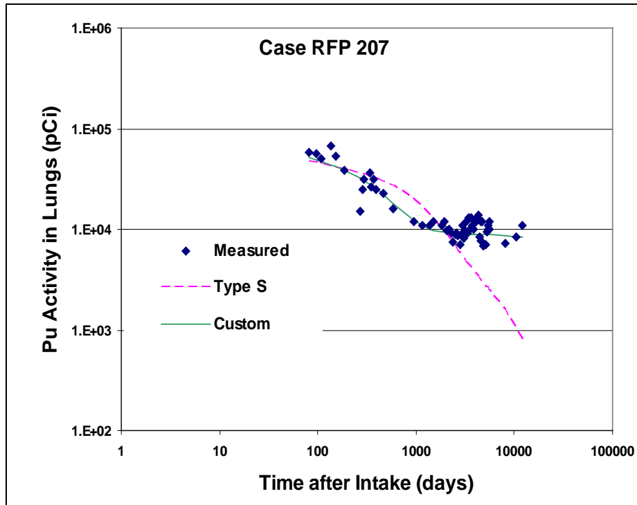
Figure A-2. Comparison of Type S and custom models for Case RFP 207.
