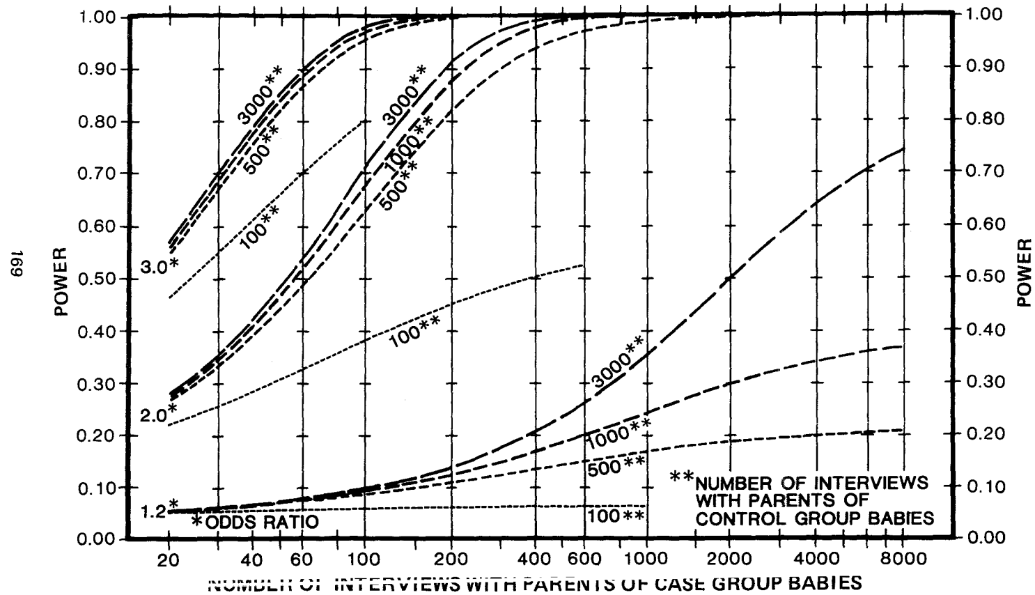
FIGURE 2. Power of the 1 Degree of Freedom Chi-Square Test, 2-Tailed, Uncorrected, Alpha = 0.05, Case-Control Study. Prevalence of Vietnam Service Among Fathers of Control Group Babies = 10%
