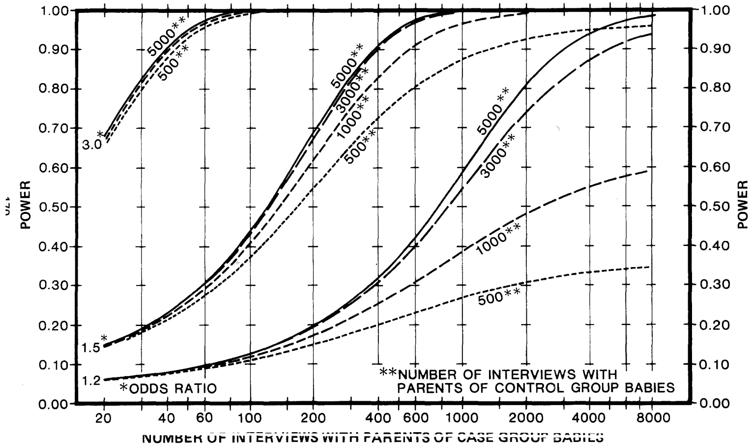
FIGURE 3. Power of the 1 Degree of Freedom Chi-Square Test, 2-Tailed, Uncorrected, Alpha = 0.05, Case-Control Study. Prevalence of Vietnam Service Among Fathers of Control Group Babies = 20%
