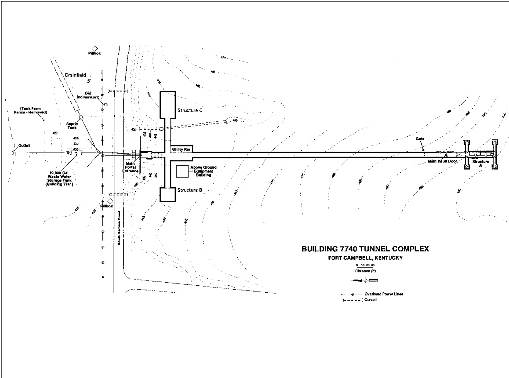
Figure 2-1. General plan view of ABC Structure.
