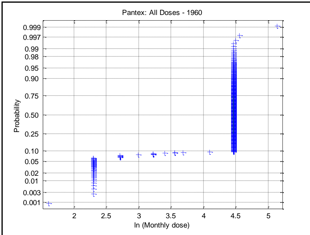
Figure 6-3. Log probability plot of Pantex dosimetry data that includes missed doses.
