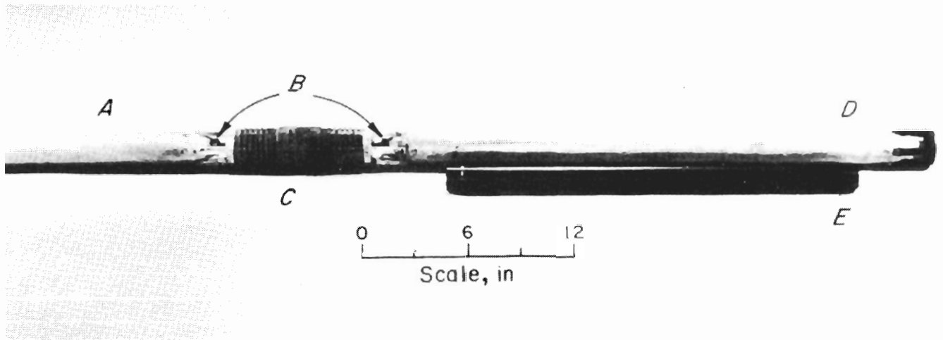
Figure A-3.-Sensor package and canister. A, Electronics; B, 3/16-in-OD steel conduit; C, sensor-electronics transition piece; D, sensor canister; E, sensor.
