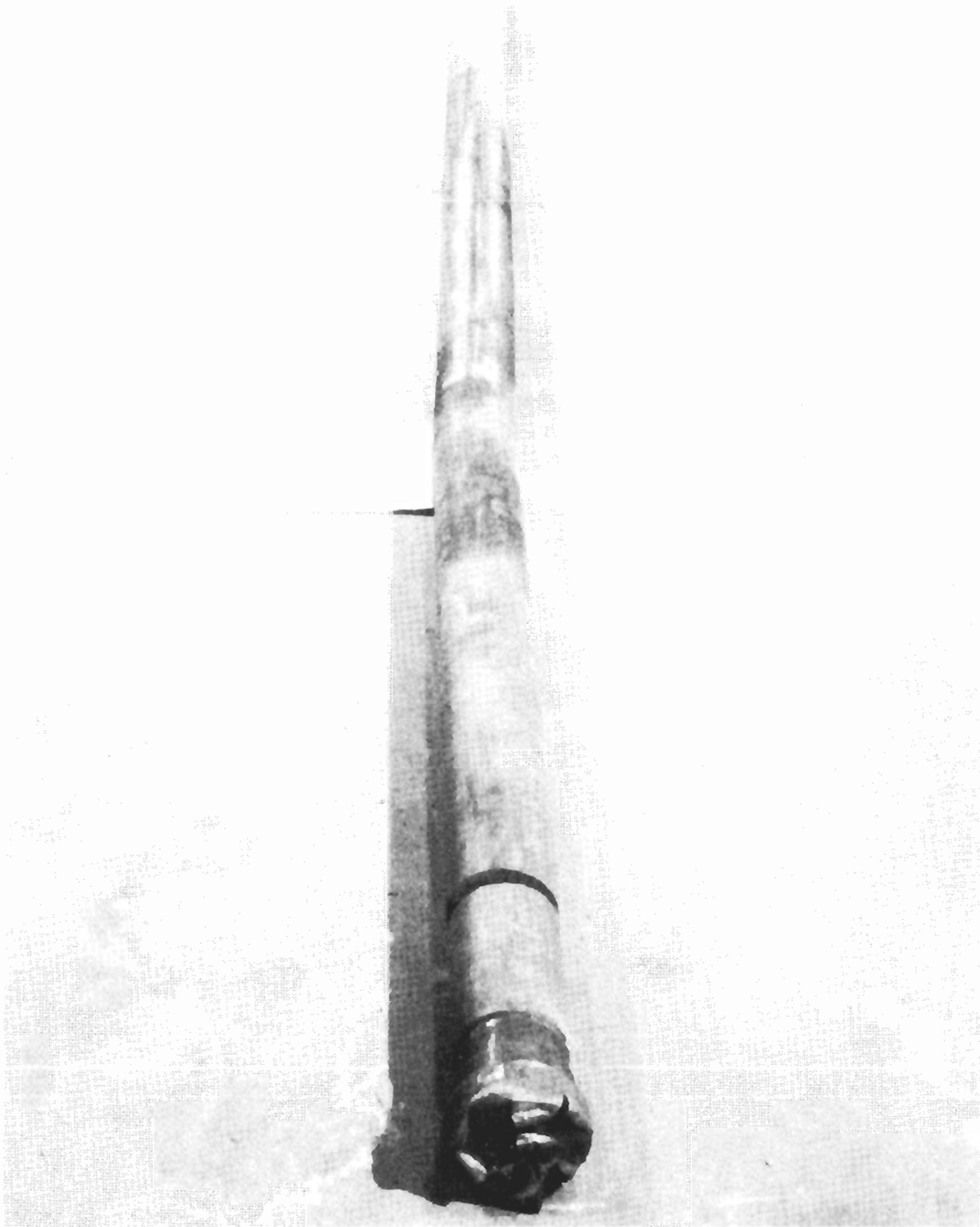
Figure 6.-Downhole motor (shown equipped with 2° bent housing and polycrystalline diamond cutter bit, although 1° bent housing used during in-mine test).
