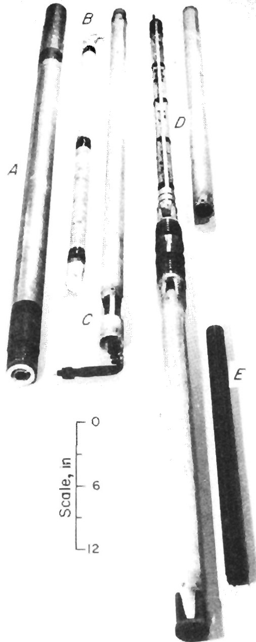
Figure 2.—Downhole guidance probe. A, Transmitter; B, batteries and canister; C, battery-transformer cable; D, electronics and canister; E, sensor package and canister.
