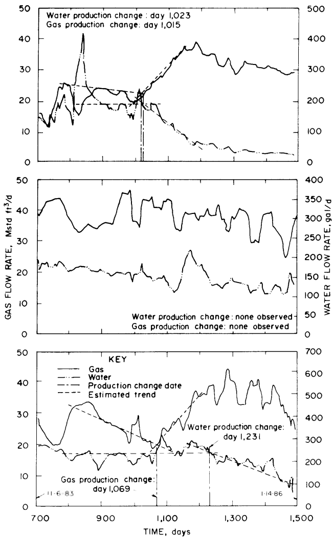
Figure 9.-Daily gas and water production rates for pattern wells 14 (top), 15 (middle), and 16 (bottom).
