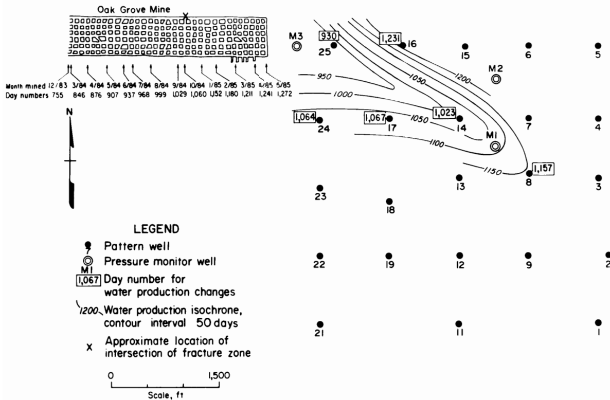
Figure 14.—Isochrone map for mining-induced water production changes.
