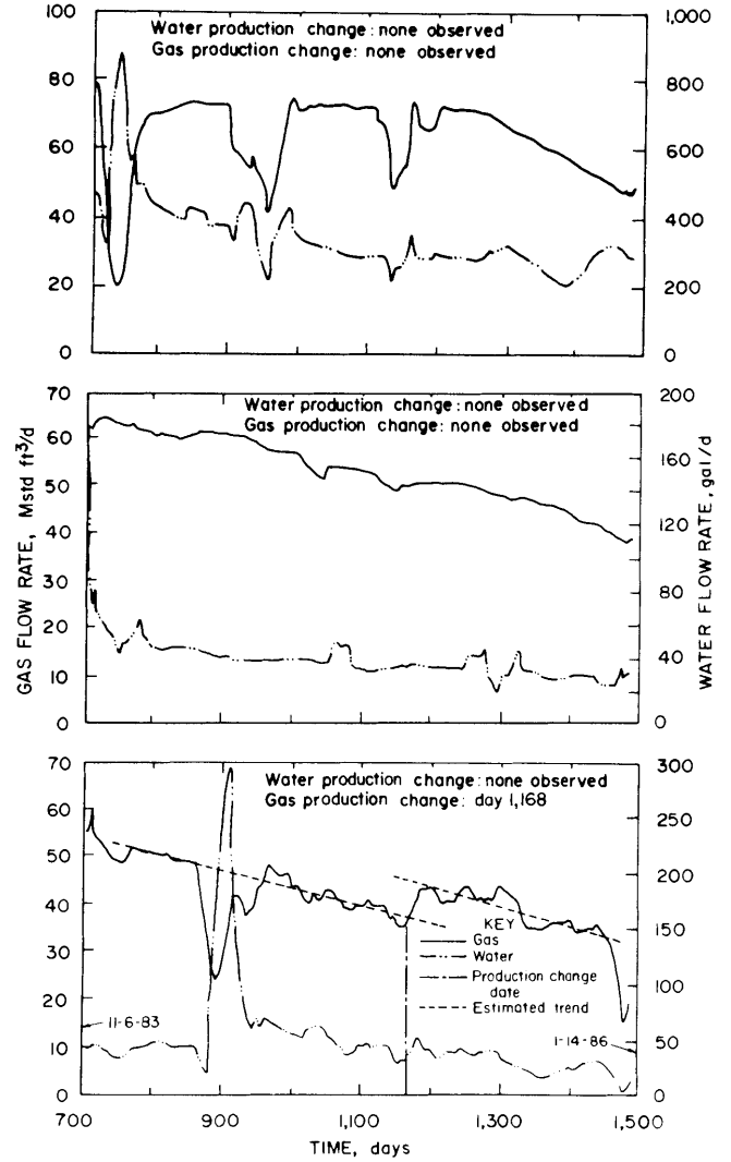
Figure 8.-Daily gas and water production rates for pattern wells 11 (top), 12 (middle), and 13 (bottom).
