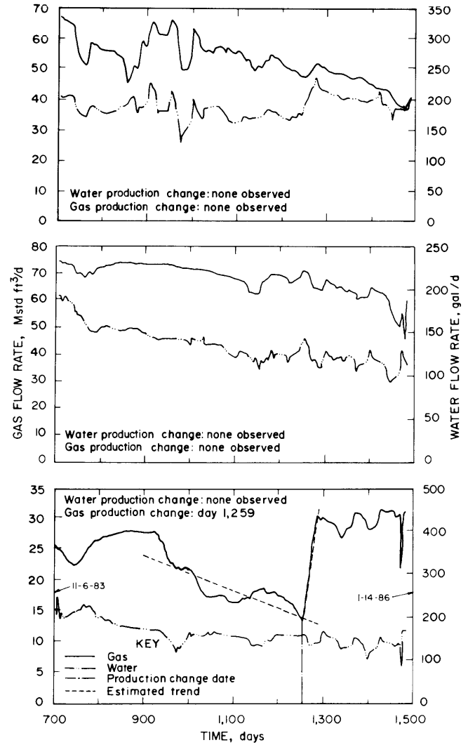
Figure 6.—Daily gas and water production rates for pattern wells 4 (top), 5 (middle), and 6 (bottom).
