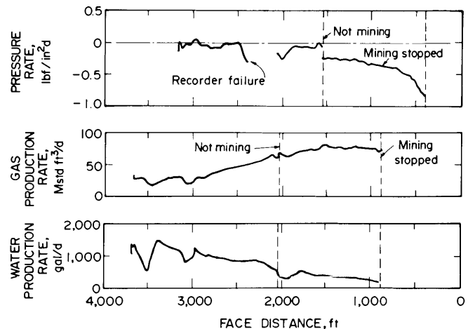
Figure 16.—Graph of water and gas production rates, and pressure rates versus face position for monitor well M3 and pattern well 25.
