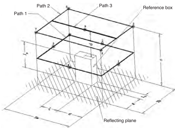
Figure 1—Example of reference and measurement parallelepiped surfaces. • Microphones
