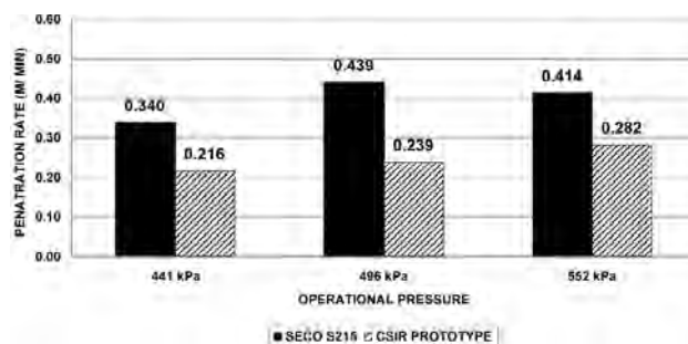
Figure 6—Performance comparisons while drilling in concrete
