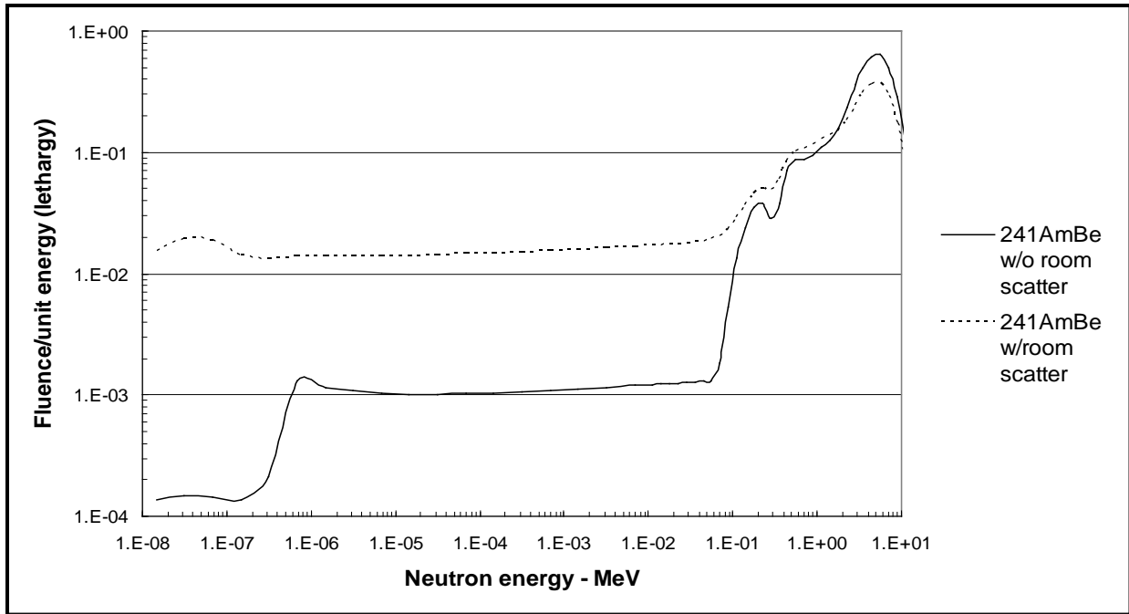
Figure A-9. Lethargy neutron spectra for an 241 AmBe calibration source with and without room scatter (IAEA 2001).
