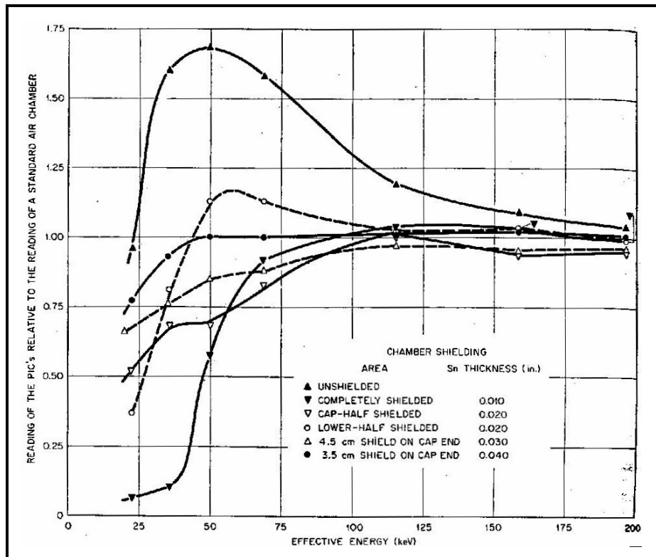
Figure 6-4. X-ray energy dependence of PICs (Sanders, Auxier, and Cheka 1959).
