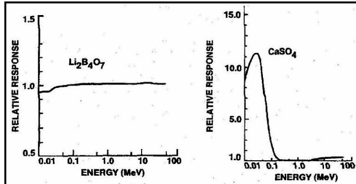
Figure A-1. Typical photon energy response curves for Li 2 B 4 O 7 and CaSO 4 TLD elements (Allen and Schoengold 1995).
