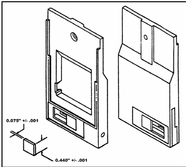
Figure 6-2. REECo badge holder (REECo 1990).
