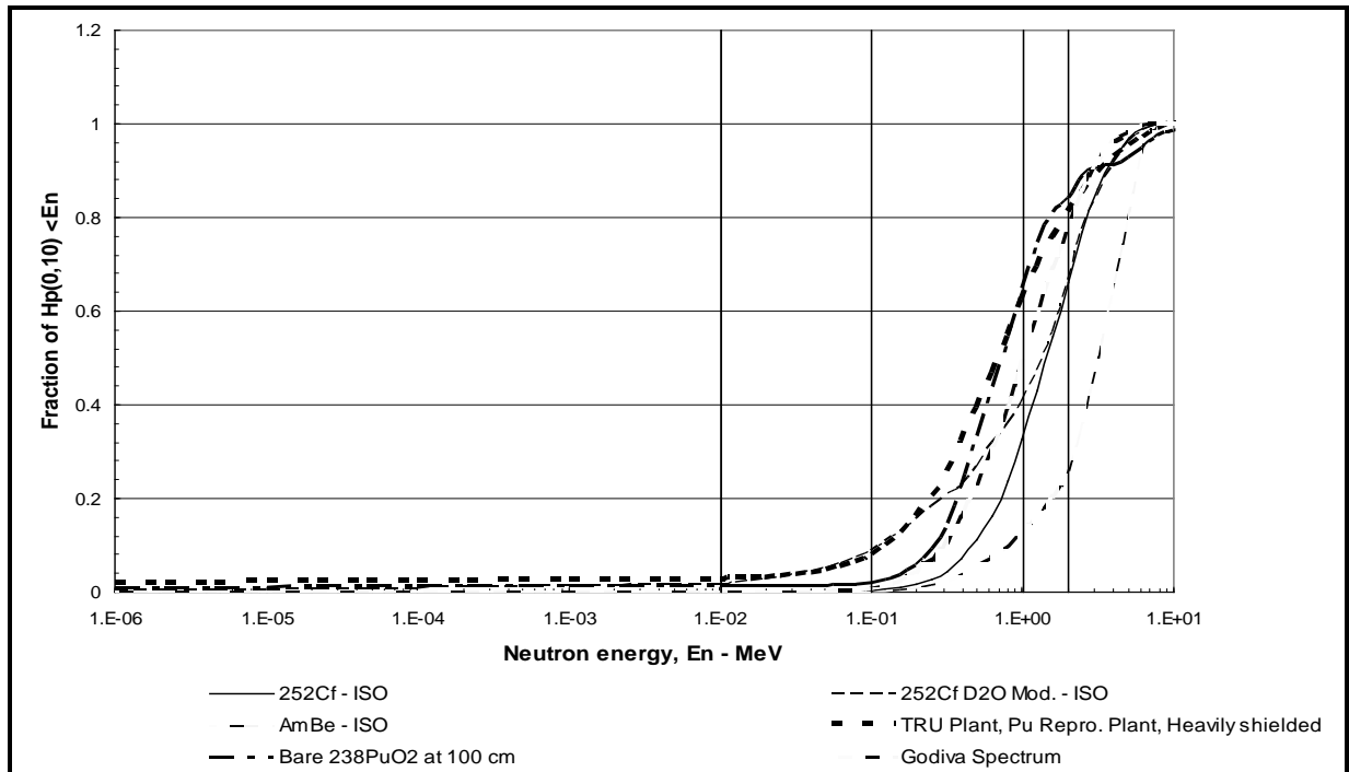
Figure A-10. Fraction of H_p(10,0) due to neutrons with energies less than E_n .
