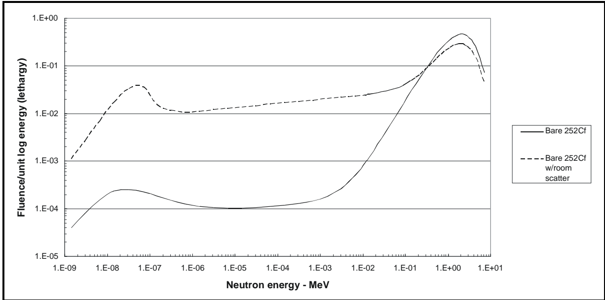
Figure A-7. Lethargy neutron spectra for 252 Cf calibration source with and without room scatter (IAEA 2001).
