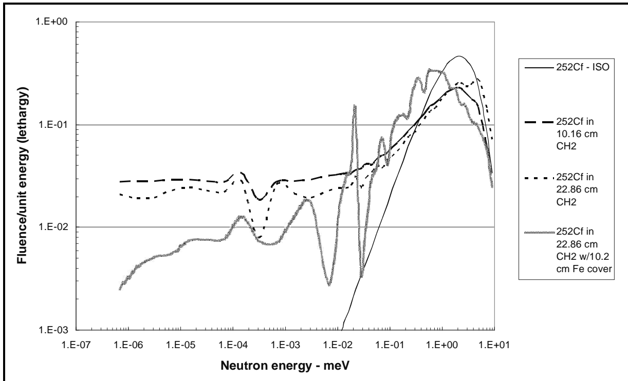
Figure A-8. Lethargy neutron spectra for 252 Cf with various thickness moderators (IAEA 2001).
