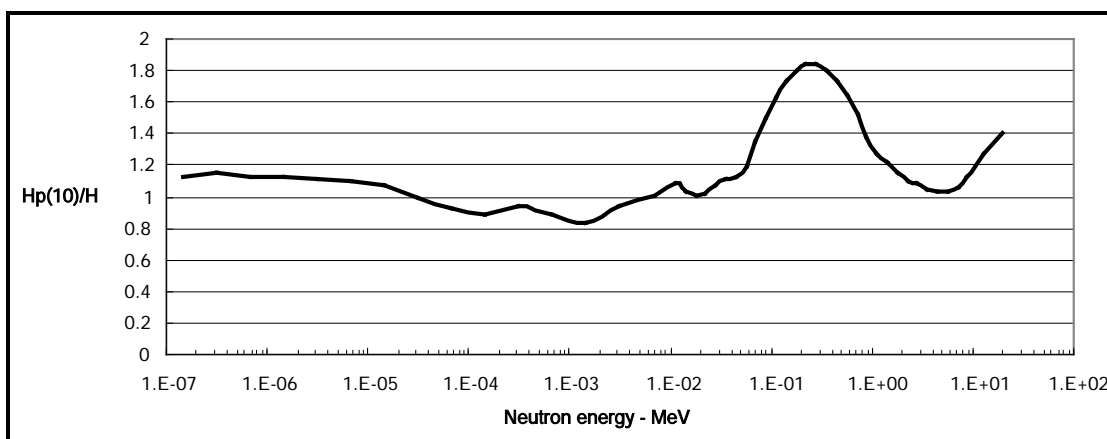
Figure 6-6. Ratio of fluence to dose conversion coefficients for personal dose equivalent H_p(10, 0^\circ) to conversion coefficients for dose equivalent H
