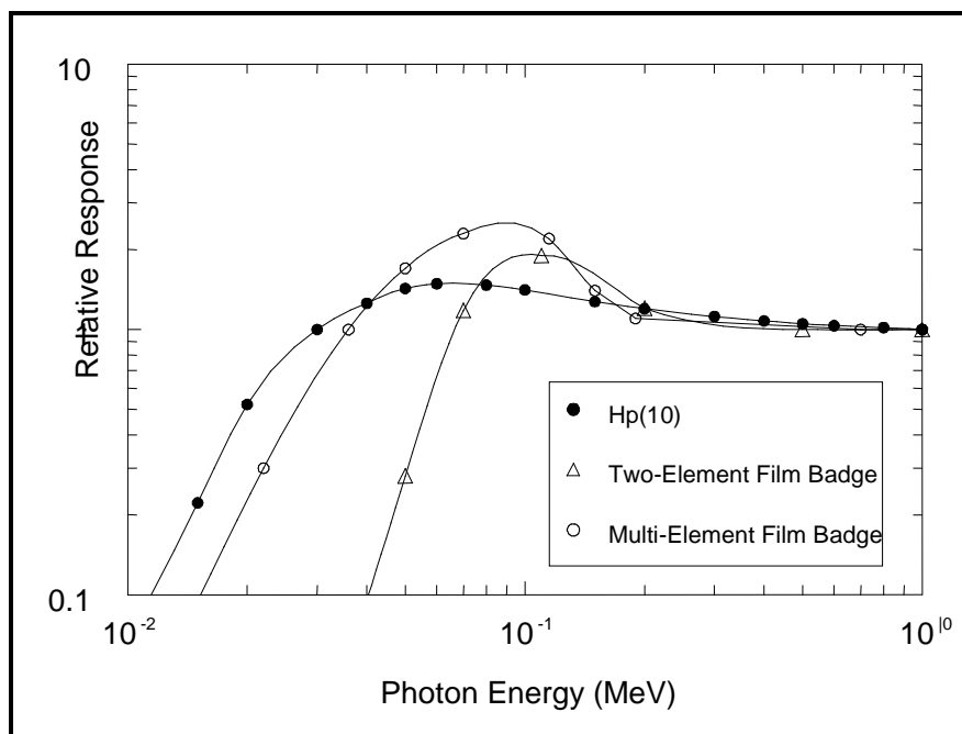
Figure 6-1. Comparison of Hp(10) for photons with energy responses for sensitive DuPont 502 emulsion in two-element film badge (Pardue, Goldstein, and Wollan 1944) and sensitive DuPont 555 emulsion in multi-element film badge (Thornton, Davis, and Gupton 1961).
