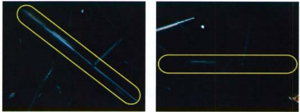
Figure 14. Field of View: 0.5mm; Parallel extinction.
