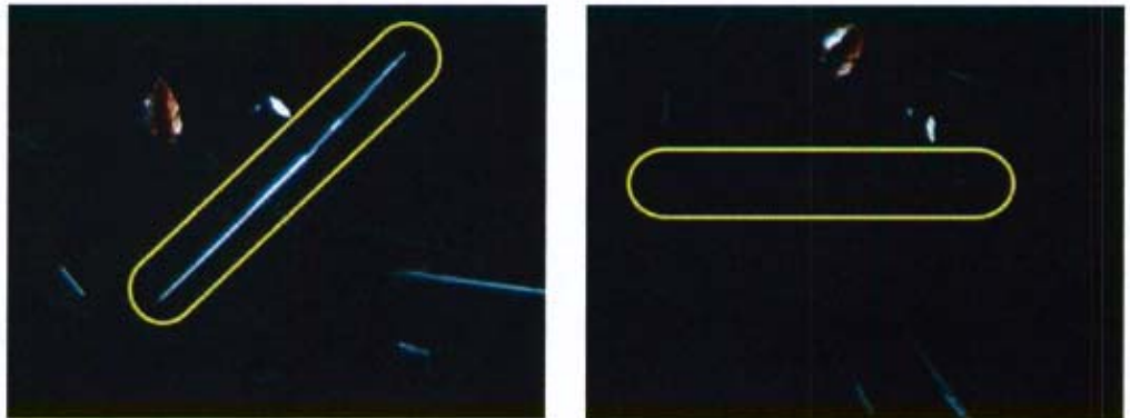
Figure 15. Field of View: 1.0mm; Parallel extinction.
