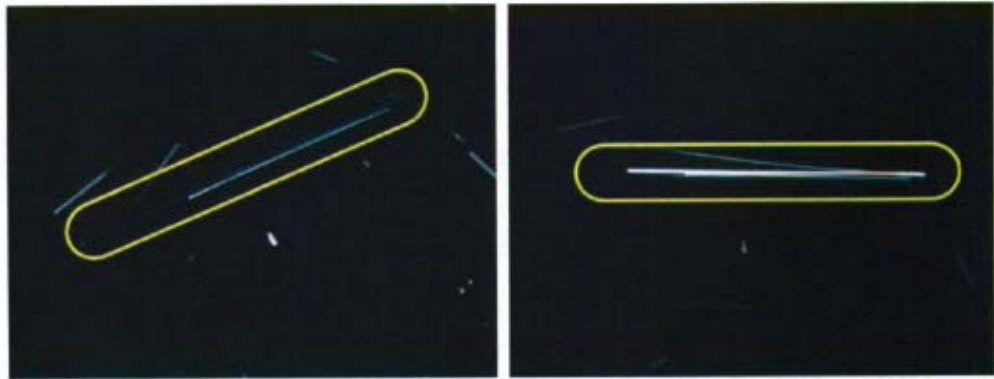
Figure 155. Field of View: 1.0mm; 24 degree extinction angle.
