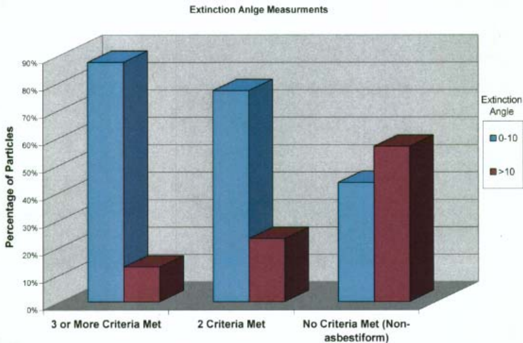
Figure 1. Chart showing the percentage of particles with extinction angles less than and greater than ten degrees for each category.
