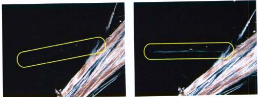
Figure 22. Field of View: 2.5mm; 12 degree extinction angle.
