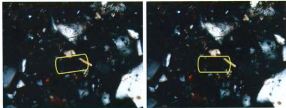
Figure 145. Field of View: 0.5mm; 7 degree extinction angle.
