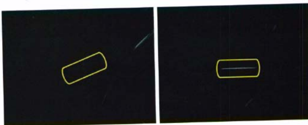
Figure 121. Field of View: 0.5mm; 22 degree extinction angle.
