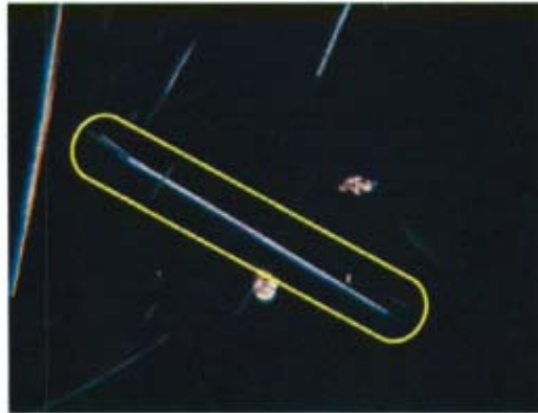
Figure 23. Field of View: 4.0mm; Parallel extinction.
