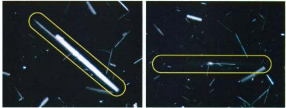
Figure 63. Field of View: 0.5mm; Parallel extinction.
