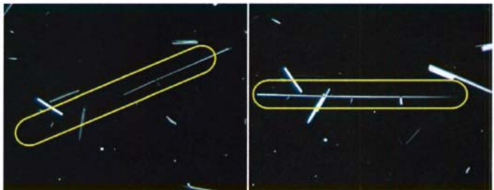
Figure 81. Field of View: 1.0 mm; Parallel extinction.
