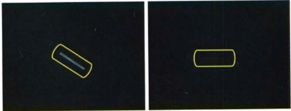
Figure 102. Field of View: 0.5mm; Parallel extinction.
