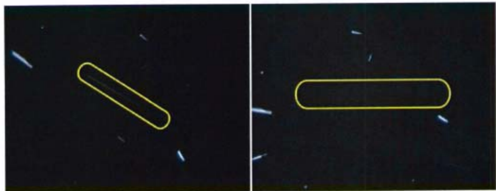
Figure 75. Field of View: 0.5mm; Parallel extinction.
