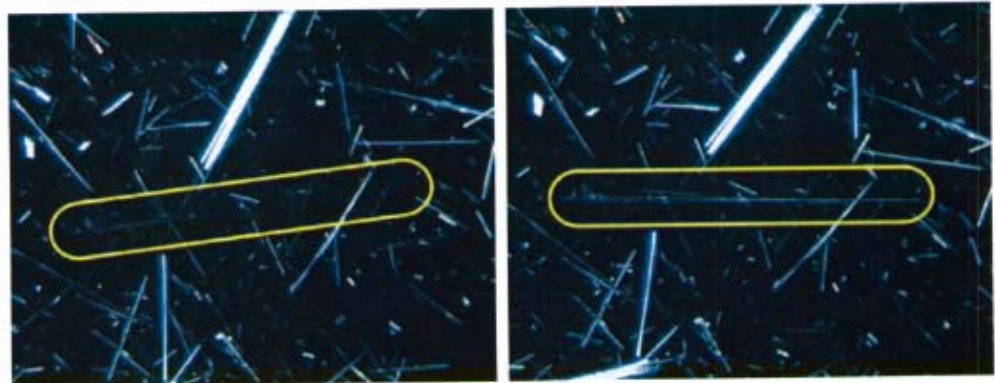
Figure 65. Field of View: 1.0mm; 7 degree extinction angle.
