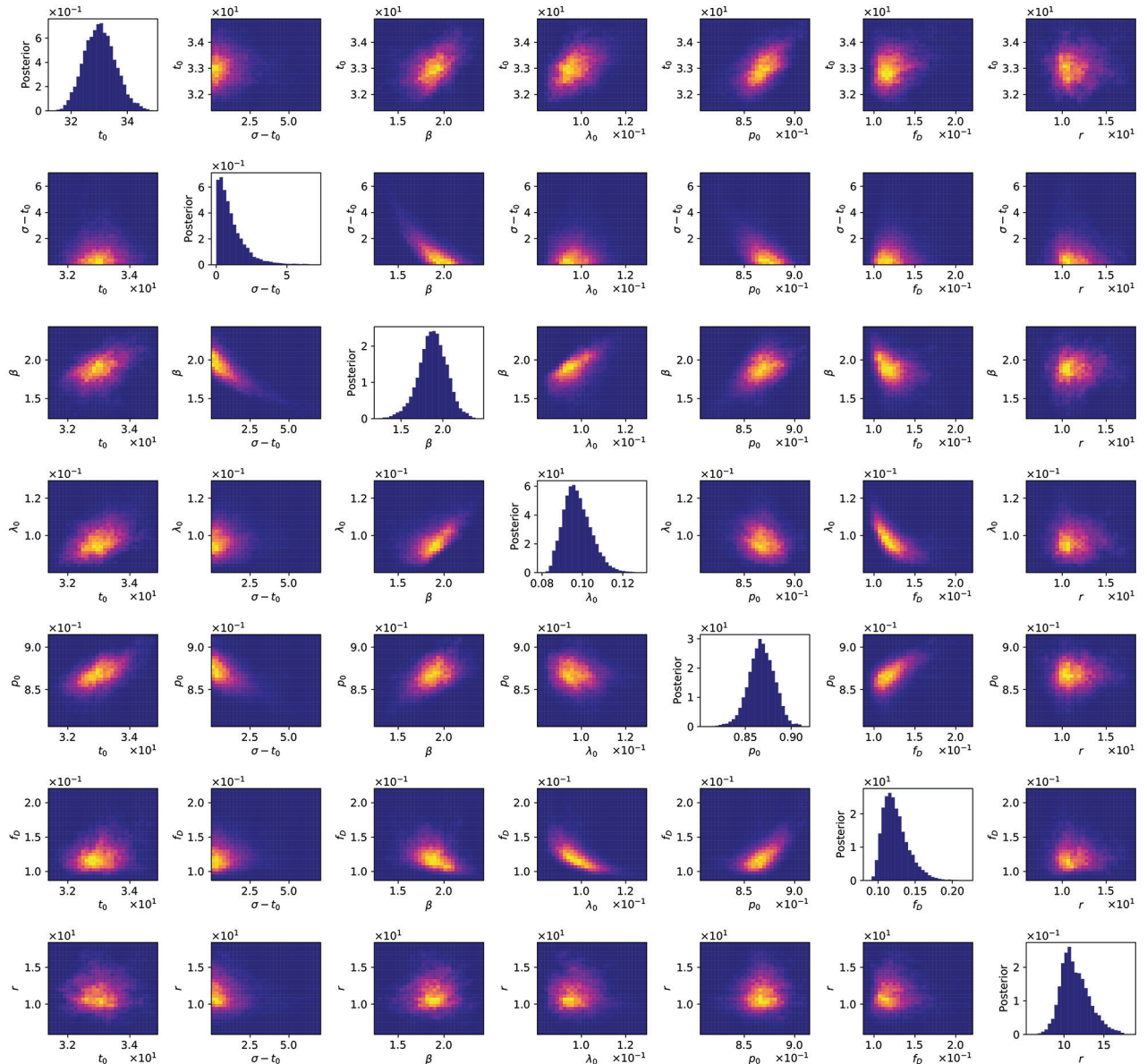
Figure 6. Matrix of 1- and 2-dimensional projections of the 7-dimensional posterior samples obtained for the adjustable parameters associated with the compartmental model ( n = 0 ) for daily new case counts of coronavirus disease in the New York City, New York, metropolitan statistical area, United States, January 21–June 21, 2020. Plots of marginal posteriors (1-dimensional projections) are shown on the diagonal from top left to bottom right. Other plots are 2-dimensional projections indicating the correlations between parameter estimates. Brightness indicates higher probability density. A compact bright area indicates absence of or relatively low correlation. An extended, asymmetric bright area indicates relatively high correlation.
