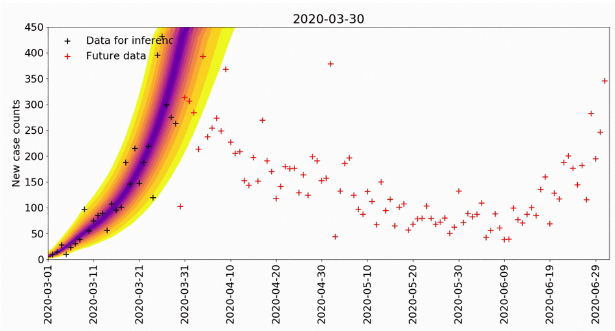
Appendix Video 6. Daily predictive inferences for new case counts of coronavirus disease in the metropolitan statistical area around Seattle, Washington, USA, March 30–June 17, 2020. Inferences are conditioned on the single-phase ( n = 0 ) compartmental model. (Video, https://wwwnc.cdc.gov/eid/images/20-3364-App-video-6.gif )
