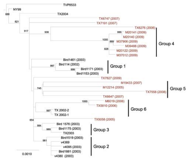
Figure 1. Maximum-likelihood phylogenetic tree of Upper Texas Gulf Coast, USA, West Nile virus isolates, 2002–2009. The tree was inferred from open reading frame sequences of 33 Upper Texas Gulf Coast isolates and NY99 by using PhyML (17) and rooted with IS-98 STD. The outgroup has been removed. Bootstrap values are for 1,000 replicates and only values >500 are shown. Groups 1–3 were previously identified by May et al. (12). Red, isolates sequenced in this study. Scale bar indicates nucleotide substitutions per site.
