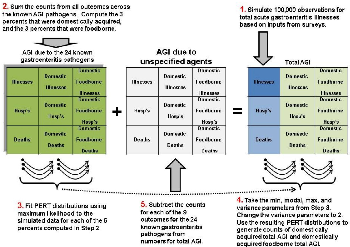
Figure 1: Schematic illustration for the method used to estimate AGI due to unspecified acute gastroenteritis agents
